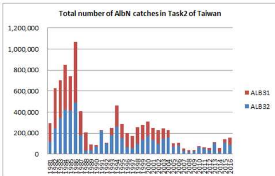
Figure 9. By ICCAT albacore sampling areas 31 and 32, yearly number of reported AlbN size measurements (Upper) and yearly number of AlbN catches reported in Task2 (Lower) of Taiwanese longline fisheries in the North Atlantic Ocean, dating from 1981 to 2016.
